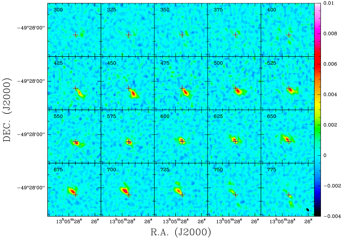
Fig. 9. \text{CH}_3\text{C}_2\text{H} 5_0 \rightarrow 4_0 channel maps. For the units of velocity, ordinate, and the wedge as well as the position of the crosses, see Fig. 3. 0.01 Jy correspond to \approx 0.42 K. The beam size is shown in the lower right corner of the figure.
