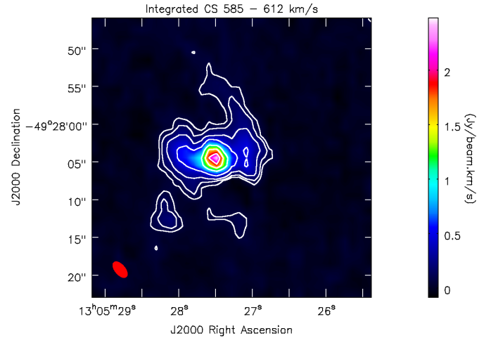
Fig. 25. Primary beam corrected CS J = 2 \rightarrow 1 emission (Briggs weighting with a robustness parameter of 0.0) integrated over the velocity interval 585 - 612 \text{ km s}^{-1} , the near systemic velocity range, where nuclear absorption is not as strong as at adjacent velocities. Contours: 0.025, 0.05, 0.1, 0.2, 0.4, 0.6, and 0.8 times the integrated peak flux density of 2.48 \text{ Jy km s}^{-1} \text{ beam}^{-1} . Overall, line absorption plays a lesser role than in Fig. 24. While the southern region of enhanced emission is part of the southeastern arm, the hotspot around 7'' farther to the east is (as in Fig. 24) a separate feature, possibly related to Marconi et al.'s (2000) Knot B (Sect. 4.1.3).
