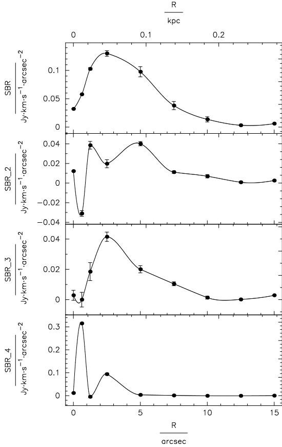
Fig. 18. Final parametrisation: surface brightness. Negative values might reflect statistical errors, but might also be due to absorption. From top to bottom: c-C 3 H 2 J = 2_{12} \rightarrow 1_{10} (SBR), CH 3 C 2 H 5_0 \rightarrow 4_0 (SBR-2) and, overlapping, c-C 3 H 2 J = 4_{32} \rightarrow 4_{23} (SBR-3) and H42 \alpha (SBR-4; see Table 1 for details to the transitions). The abscissa provides galactocentric radii and the ordinate displays emission in units of Jy km s -1 arcsec -2 . Further information is given in Sect. 4.6.2.
