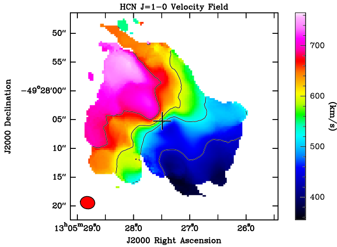
Fig. 11. The HCN J = 1 \rightarrow 0 moment 1 velocity field, clipped at the 5\sigma level. Contours are 440, 520, 600, and 680 \text{ km s}^{-1} from lower right to upper left. Primary beam correction and Briggs weighting (robustness parameter +2.0) has been applied. The restored beam ( 2''.52 \times 2''.17 , PA = 78^\circ ) is shown in the lower left corner of the image. The cross indicates the \lambda \approx 3 \text{ mm} radio continuum peak.
