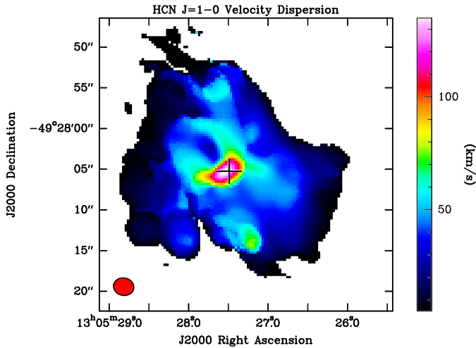
Fig. 13. A map of the HCN J = 1 \rightarrow 0 moment 2 velocity dispersion, clipped at the 5\sigma level. Primary beam correction and Briggs weighting (robustness parameter +2.0) has been applied. The restored beam ( 2''.52 \times 2''.17 , PA = 78^\circ ) is shown in the lower left corner of the image. The cross indicates the \lambda \approx 3 mm radio continuum peak, while the position of the secondary maximum in the south (also seen in Fig. 14) is inconspicuous in all other aspects.
