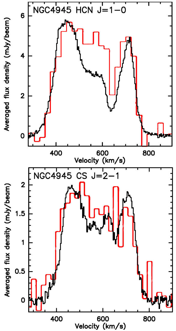
Fig. 5. Upper panel, black: HCN J=1\rightarrow 0 spectrum with a channel spacing of 3.3 \text{ km s}^{-1} from the central 0.25 \text{ arcmin}^2 of NGC 4945. The covered area is limited by \alpha_{J2000} = 13^{\text{h}} 05^{\text{m}} 26^{\text{s}} and 13^{\text{h}} 05^{\text{m}} 29^{\text{s}} and by \delta_{J2000} = -49^\circ 28' 50'' and -49^\circ 28' 20'' . The ordinate displays unweighted average values from pixels of the entire area (moment -1 ) as a function of barycentric velocity in units of \text{mJy beam}^{-1} . For spatially integrated flux densities, multiply by 200 \pm 20 . Lower panel, black: A CS J=2\rightarrow 1 spectrum with a channel spacing of 3.0 \text{ km s}^{-1} from the same region. Ordinate and abscissa: same units as for HCN. For spatially integrated flux densities, multiply by 240 \pm 24 . Overlaid spectra (red) with lower velocity resolution and larger beam size ( \approx 1' ), matched to the amplitude of our spectra, are taken from Wang et al. (2004).
