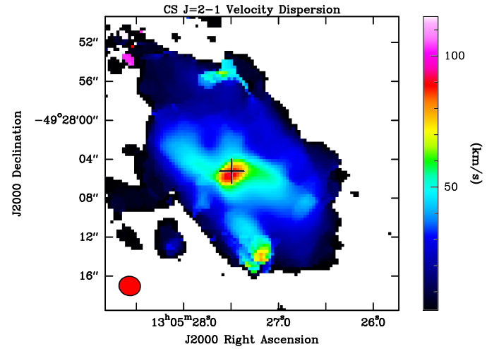
Fig. 14. A map of the CS J = 2 \rightarrow 1 moment 2 velocity dispersion, clipped at the 5\sigma level. Primary beam correction and Briggs weighting (robustness parameter +2.0) has been applied. The restored beam ( 2''.22 \times 1''.99 , PA = 79^\circ ) is shown in the lower left corner of the image. The cross indicates the \lambda \approx 3 mm radio continuum peak, while the secondary peak in the south (also seen in Fig. 13) is inconspicuous in all other aspects.
