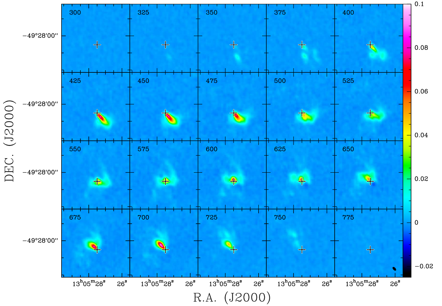
Fig. A.2. ^{12}\text{C}^{32}\text{S} (CS) J = 2 \rightarrow 1 channel maps. For the units of velocity, ordinate, and the wedge as well as for the position of the crosses, see Fig. 3. 0.1 Jy correspond to \approx 3.3 K. The beam size is shown in the lower right corner of the figure.
