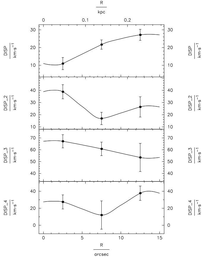
Fig. 21. Final parametrization: Intrinsic dispersion (see Sect. 4.6.1) as a function of galactocentric radius (this may be compared with Fig. 16). From top to bottom as in Fig. 18: c\text{-C}_3\text{H}_2 (DISP), \text{CH}_3\text{C}_2\text{H} (DISP-2) and, overlapping, c\text{-C}_3\text{H}_2 (DISP-3) and \text{H}42\alpha (DISP-4; see Table 1).
