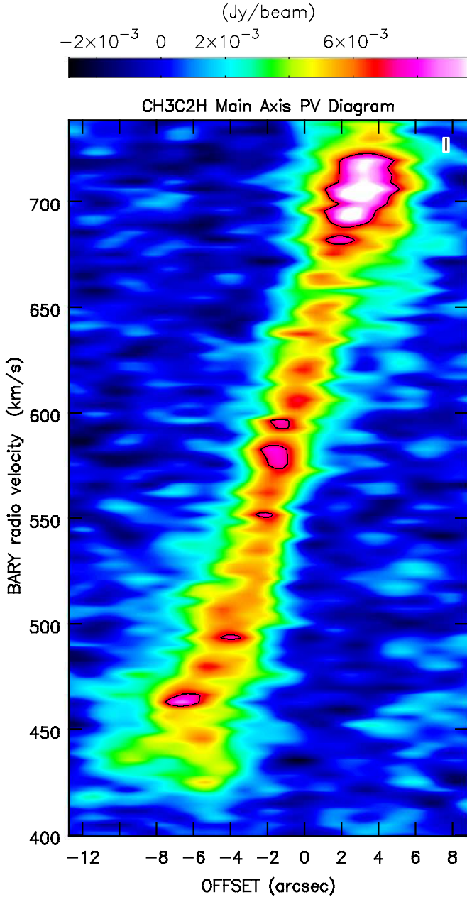
Fig. 17. Position-velocity plot of \text{CH}_3\text{C}_2\text{H} 5_0 \rightarrow 4_0 along the major axis with the abscissa scaled relative to the continuum peak. Contour: 7 \text{ mJy beam}^{-1} . The plot emphasizes (a) the clumpiness of the gas, (b) the steepening of the rotation curve between barycentric V \approx 500 \text{ km s}^{-1} and the systemic velocity of V \approx 571 \text{ km s}^{-1} and (c) its flattening between 470 and 500 \text{ km s}^{-1} .
