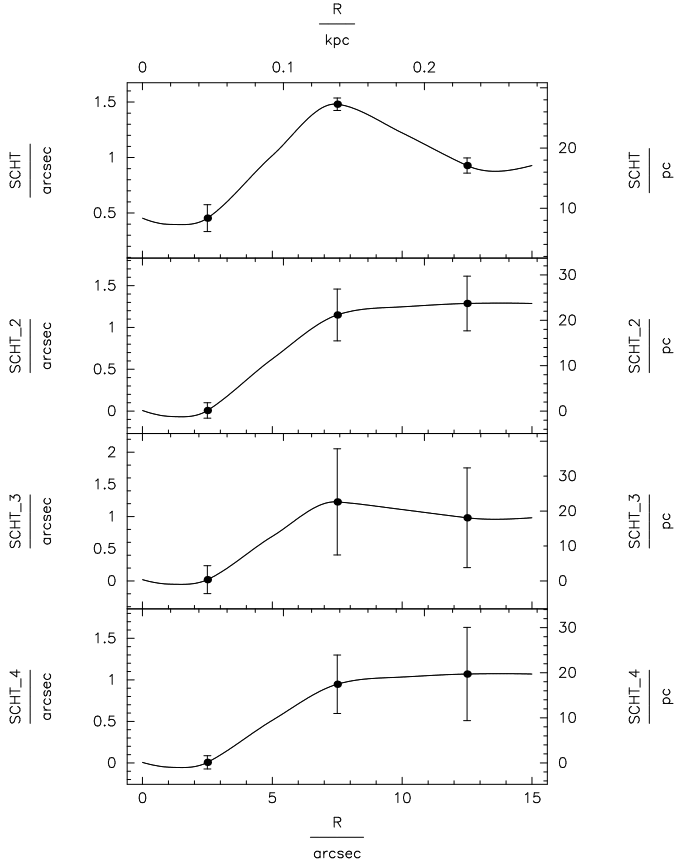
Fig. 20. Final parametrization: full scale height. From top to bottom in the same order as in Fig. 18: c\text{-C}_3\text{H}_2 (SCHT), \text{CH}_3\text{C}_2\text{H} (SCHT-2) and, overlapping, c\text{-C}_3\text{H}_2 (SCHT-3) and \text{H}42\alpha (SCHT-4). Ordinate on the left hand side: scale height in arcseconds; ordinate on the right hand side: scale height in pc, both as a function of galactocentric radius.
