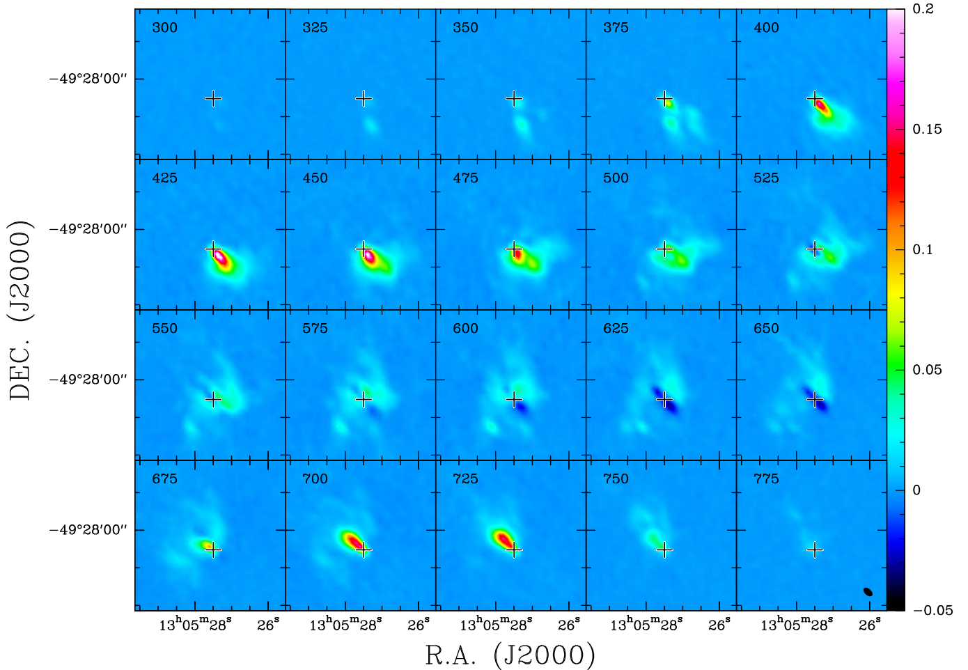
Fig. 3. \text{H}^{12}\text{C}^{14}\text{N} (HCN) J=1\rightarrow 0 channel maps with the crosses indicating (as in case of Figs. 7, 9, A.1, A.2, and A.3) the position of the radio continuum peak. The spacing between tick-marks along the y-axis corresponds to 10'' . Central barycentric velocities in \text{km s}^{-1} are given in the upper left corners of each map. The systemic velocity is near 571 \text{ km s}^{-1} (Sect. 2). The wedge provides intensities in units of \text{Jy beam}^{-1} . Note the dark areas between 525 and 650 \text{km s}^{-1} , where the line is seen in absorption. The large scale rotation of the highly inclined galaxy is such that emission at low velocities is mainly originating from the southwest of the center, while high velocity emission arises from the northeast. 0.1 Jy correspond to \approx 4.0 \text{ K} main beam brightness temperature. 1'' represents a projected linear scale of 19 pc. The beam size is shown in the lower right corner of the figure.
