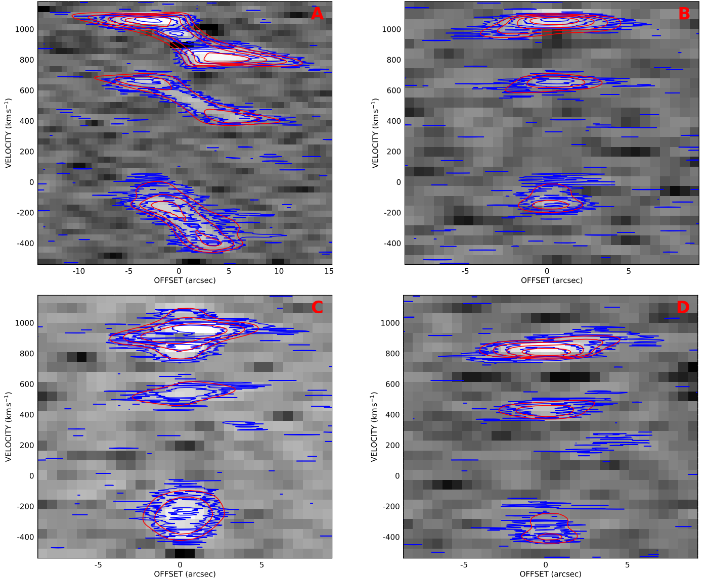
Fig. 23. PV-diagrams along the lines shown in Fig. 22, each with (from top to bottom) \text{c-C}_3\text{H}_2 2_{12} \rightarrow 1_{01} , \text{CH}_3\text{C}_2\text{H} 5_0 \rightarrow 4_0 and, overlapping, \text{C}_3\text{H}_2 4_{32} \rightarrow 4_{23} and \text{H}42\alpha . The velocity scale refers to that of the \text{CH}_3\text{C}_2\text{H} line (see Sect. 4.6.2 and Table 1). Dark: low intensity; light grey: high intensity. Top left panel: cut A (see also Fig. 22) along the major axis from the northeast toward the southwest. Top right panel: cut B perpendicular to the major axis crossing the 710 \text{ km s}^{-1} peak from the southeast toward the northwest. Bottom left panel: cut C perpendicular to the major axis, central line. Bottom right panel: cut D perpendicular to the major axis crossing the 430 \text{ km s}^{-1} peak. A, B, C or D are displayed in the upper right corner of their respective panels. Blue contours: original data cube. Red contours: model data cube with constant vertical gradient in radial motion and final rotation curve (see top two panels of Fig. 19). Contours: 0.1, 0.2, 0.4, 0.8 \text{ mJy beam}^{-1} .
