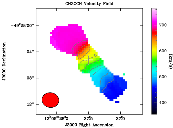
Fig. 15. The \text{CH}_3\text{C}_2\text{H} 5_0 \rightarrow 4_0 velocity field, clipped at the 5\sigma level. Unlike in Figs. 11 and 12, here the emission is confined to the nuclear disk. Primary beam correction and Briggs weighting (robustness parameter +2.0) has been applied. The contours start at 470 \text{ km s}^{-1} and reach 695 \text{ km s}^{-1} ; their spacing is 25 \text{ km s}^{-1} . The restored beam ( 2''.65 \times 2''.28 , \text{PA} = 80^\circ ) is shown in the lower left corner of the image. The cross indicates the \lambda \approx 3 \text{ mm} radio continuum peak.
