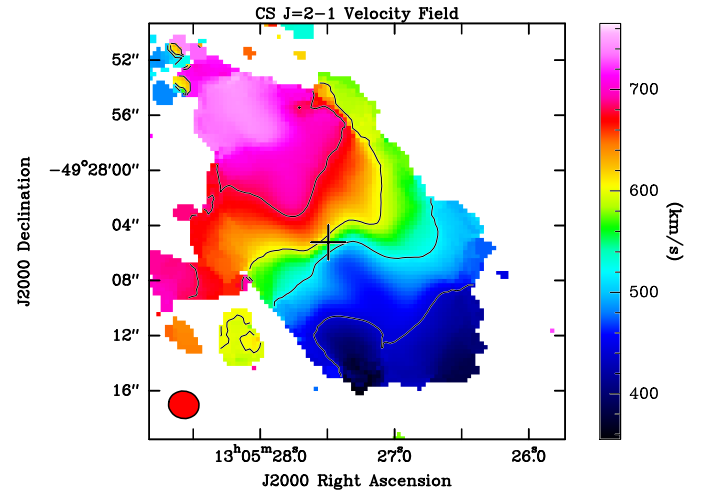
Fig. 12. The CS J = 2 \rightarrow 1 moment 1 velocity field, clipped at the 5\sigma level. Contours are 440, 520, 600, and 680 \text{ km s}^{-1} from lower right to upper left. Primary beam correction and Briggs weighting (robustness parameter +2.0) has been applied. The restored beam ( 2''.22 \times 1''.99 , PA = 78^\circ ) is shown in the lower left corner of the image. The cross indicates the \lambda \approx 3 \text{ mm} radio continuum peak.
