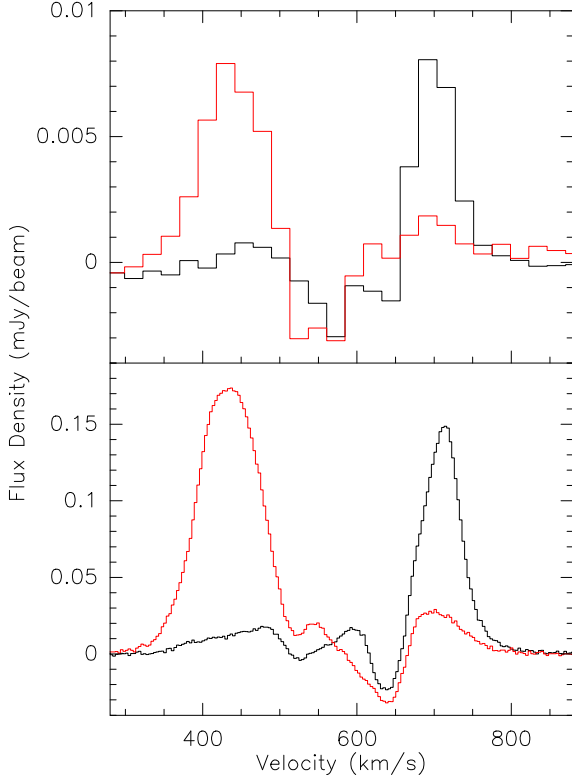
Fig. 6. Lower panel: HCN J = 1 \rightarrow 0 spectra with a channel spacing of 3.3 \text{ km s}^{-1} . Black: spectrum from the northeastern region (peak near V = 710 \text{ km s}^{-1} ) showing absorption. Red: spectrum from the southwestern region (peak near V = 430 \text{ km s}^{-1} ) showing absorption. The separation between the two regions is the line perpendicular to the nuclear disk crossing the peak of the radio continuum emission (see Figs. 2 and 3). Upper panel: The same for \text{H}^{13}\text{CN } J = 1 \rightarrow 0 , but with a channel width of 24 \text{ km s}^{-1} . The ordinate provides average flux densities per beam over the covered area. The galaxy’s systemic velocity is close to V = 571 \text{ km s}^{-1} .
