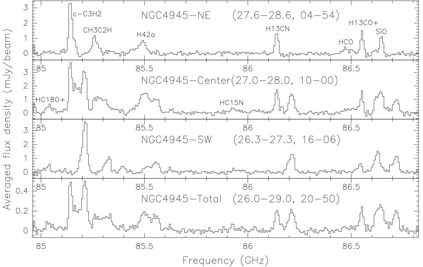
Fig. 8. Spectra from the broad \text{HC}^{15}\text{N} window with seven contiguous channels smoothed, yielding a channel spacing of \approx 23 \text{ km s}^{-1} . The molecular species related to detected spectral features are given in the two top panels and are described in more detail in Table 1. For \text{H}42\alpha , see Bendo et al. (2016). Because almost 2 GHz are covered, leading to a complex correlation between velocity and frequency, amplitudes are presented as a function of observed frequency. The lowest panel presents a spectrum from the central 0.25 \text{ arcmin}^2 , similar to the spectra shown in Fig. 5. The three upper panels show spectra from smaller areas, visualized by dashed white lines in Fig. 2, and include (from top to bottom) regions to the northeast of the center, close to the nucleus, and to the southwest of the center. The four numbers in parenthesis on the right hand side of each of these designations provide the eastern and western edge (in time seconds of Right Ascension) and the southern and northern edge (in arcseconds of Declination) of the chosen area (compare with the moment 0 maps of Figs. 2 and 4). The ordinate displays unweighted average flux densities per beam size for all pixels in the given areas, so that the values for the largest region (lowest panel), encompassing most areas with weak (or even absent) emission, are smallest. Multiply by 40 \pm 4 (upper three panels) and 250 \pm 25 to obtain spatially integrated flux densities. Applied pixel size: 1'' \times 1'' .
