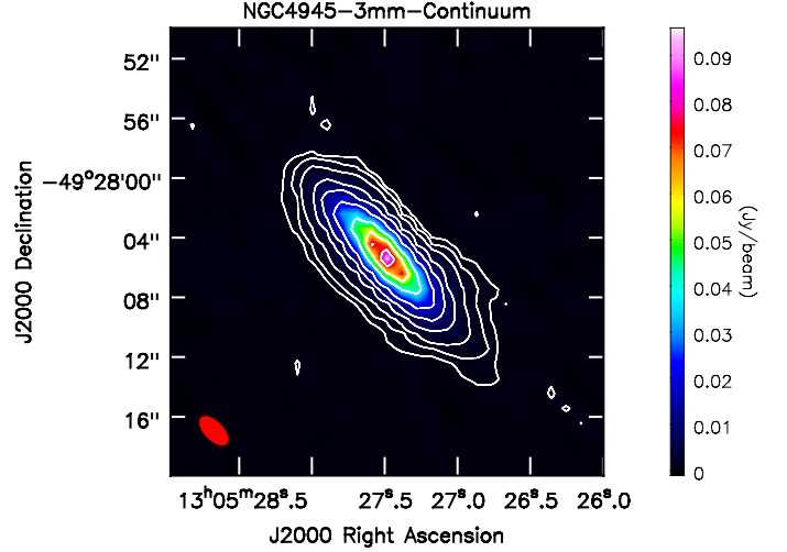
Fig. 1. An image of the \lambda \approx 3 mm continuum emission from the central region of NGC 4945 (1'' corresponds to a projected linear scale of \approx 19 pc). The map is based on the line-free sky frequencies of 88.27–88.38 GHz and 88.54–88.70 GHz in the H 12 C 14 N window, 85.60–86.01 GHz and 86.28–86.42 GHz in the H 12 C 15 N window, 97.35–97.72 GHz and 98.01–98.24 GHz in the CS window, and 100.15–100.46 GHz in the continuum window (see Sect. 2). The beam size is 2''.55 \times 1''.34 ( 0.1 \text{ Jy beam}^{-1} is equivalent to \approx 6.8 K) with a position angle of 44^\circ.2 . Contour levels are 0.5, 1, 2, 5, 10, 20, 40, 60, and 80% of the peak flux density of 96 \text{ mJy beam}^{-1} . The restored beam is shown in the lower left corner. In view of the limited extent of the emission, no primary beam correction has been applied.
