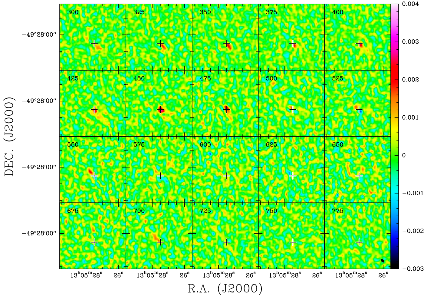
Fig. A.1. \text{H}^{12}\text{C}^{15}\text{N} ( \text{HC}^{15}\text{N} ) J = 1 \rightarrow 0 channel maps. For the units of velocity, ordinate, and wedge as well as the position of the crosses, see Fig. 3. Note that the signal seen is very close to the noise level. This or a weak transition of SO or \text{CH}_3\text{OH} may explain the “emission” at V \approx 350 \text{ km s}^{-1} . Near the systemic velocity, where the more abundant HCN isotopologues exhibit weak absorption, no signal is seen, likely also a consequence of too low signal-to-noise ratios. 0.002 Jy correspond to \approx 85 \text{ mK} . The beam size is shown in the lower right corner of the figure.
