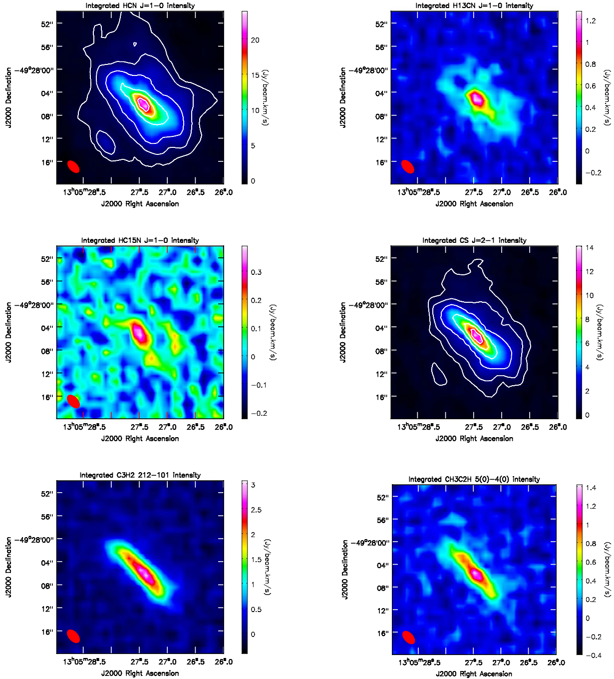
Fig. 4. Maps of primary beam corrected velocity integrated intensity (moment 0), obtained with a robustness parameter of 0.0 (Sect. 2). Data reduced with a parameter of +2.0 (close to natural weighting) do not reveal any additional features. 1'' corresponds to a projected linear scale of \approx 19 pc. Upper left: HCN J = 1 \rightarrow 0 emission with a restored beam of 2''.71 \times 1''.56 and position angle PA = 43^\circ (see the red spot in the lower left corner of the image). Contour levels: 5, 10, 20, 40, 60, and 80% of the integrated peak flux density of 24.0 \text{ Jy km s}^{-1} \text{ beam}^{-1} . Upper right: \text{H}^{13}\text{CN } J=1 \rightarrow 0 with a restored beam of 2''.72 \times 1''.57 , PA = 42^\circ . Center, left: \text{HC}^{15}\text{N } 1 \rightarrow 0 (only V > 400 \text{ km s}^{-1} ) with 2''.72 \times 1''.57 , PA = 42^\circ . Center right: CS J = 2 \rightarrow 1 . Contours: 5, 10, 20, 40, 60, and 80% of the integrated peak flux density of 14.1 \text{ Jy km s}^{-1} \text{ beam}^{-1} . Restored beam: 2''.57 \times 1''.38 , PA = 41^\circ . Lower left: \text{C}_3\text{H}_2 \text{ } 2_{12} \rightarrow 1_{01} with 2''.72 \times 1''.57 , PA = 42^\circ . Lower right: \text{C}_3\text{HC}_2\text{H } 5_0 \rightarrow 4_0 . Restored beam: 2''.72 \times 1''.57 , PA = 42^\circ . To convert \text{Jy km s}^{-1} \text{ beam}^{-1} into \text{K km s}^{-1} \text{ beam}^{-1} , multiply by \approx 37 (HCN), 39 ( \text{H}^{13}\text{CN} , \text{HC}^{15}\text{N} , \text{C}_3\text{H}_2 , and \text{CH}_3\text{C}_2\text{H} ), or 36 (CS).
