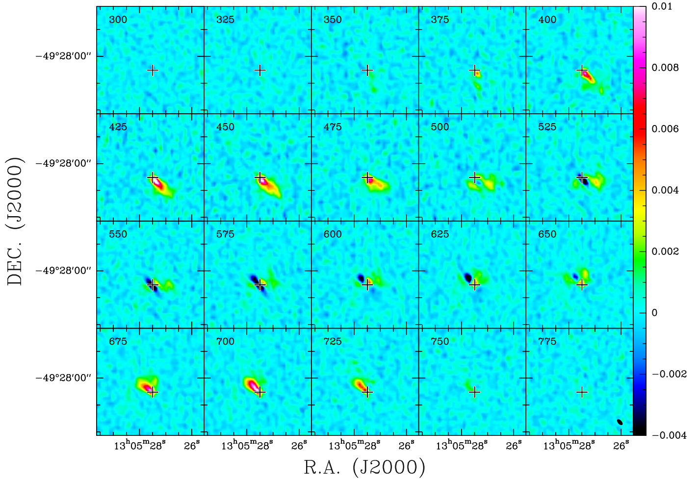
Fig. 7. \text{H}^{13}\text{C}^{14}\text{N} ( \text{H}^{13}\text{CN} ) J = 1 \rightarrow 0 channel maps. For the units of velocity, the ordinate, and the wedge as well as for the position of the crosses, see Fig. 3. As in case of the main isotopic species, absorption is present near the systemic velocities between 525 and 650 \text{km s}^{-1} . 0.01 Jy correspond to \approx 0.42 K. The beam size is shown in the lower right corner of the figure.
