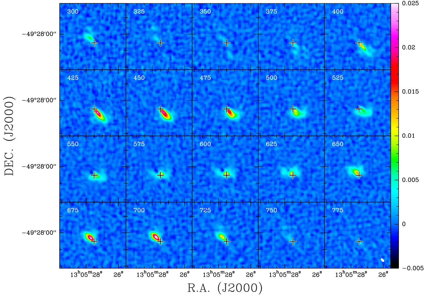
Fig. A.3. c\text{-C}_3\text{H}_2 2_{12} \rightarrow 1_{01} channel maps. For the units of velocity, ordinate, and the wedge as well as for the position of the crosses, see Fig. 3. 0.02 Jy correspond to \approx 0.85 K. The beam size is shown in the lower right corner of the figure. The emission seen at an apparent c\text{-C}_3\text{H}_2 velocity of \approx 300 \text{ km s}^{-1} is caused by the redshifted part of the \text{CH}_3\text{C}_2\text{H} J=5_0 \rightarrow 4_0 line, emitting near 710 \text{ km s}^{-1} (see also Figs. 8 and 9).
