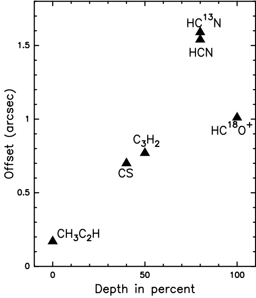
Fig. 10. Angular offsets (along the main axis with position angle 225^\circ toward the southwest) of molecular versus continuum centroid position (obtained from two-dimensional Gaussian fits) as a function of depth of the spectral dip near the systemic velocity in percent of the line peaks at V \approx 430 \text{ km s}^{-1} . The percentages given refer to a covered area of 0.25 \text{ arcmin}^2 as described in Fig. 5. Molecular species are indicated. For details, also including line assignments, formal uncertainties and rest frequencies, see Sect. 4.1.2 and Table 1).
