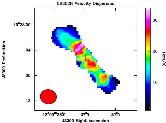
Fig. 16. A map of the \text{CH}_3\text{C}_2\text{H} 5_0 \rightarrow 4_0 velocity dispersion, clipped at the 5\sigma level. Primary beam correction and Briggs weighting (robustness parameter +2.0) has been applied. The restored beam ( 2''.65 \times 2''.28 , \text{PA} = 80^\circ ) is shown in the lower left corner of the image. The cross indicates the \lambda \approx 3 \text{ mm} radio continuum peak.
