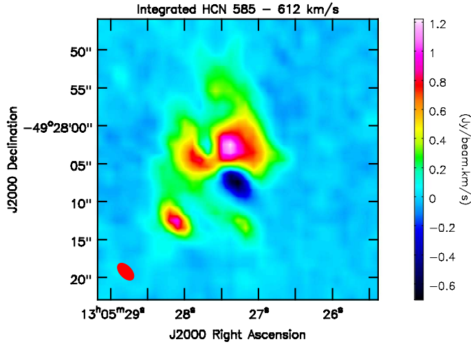
Fig. 24. Primary beam corrected HCN J = 1 \rightarrow 0 emission (Briggs weighting with a robustness parameter of 0.0) integrated over the velocity interval 585 - 612 \text{ km s}^{-1} , the near systemic velocity range, where nuclear absorption is not as strong as at adjacent velocities. The arms (mainly green color, see Sect. 4.7) are visible in the northwest and southeast, likely connected by the elongated region of strong emission along an east-west axis. See Fig. 25 for an even clearer image, where absorption plays a lesser role.
