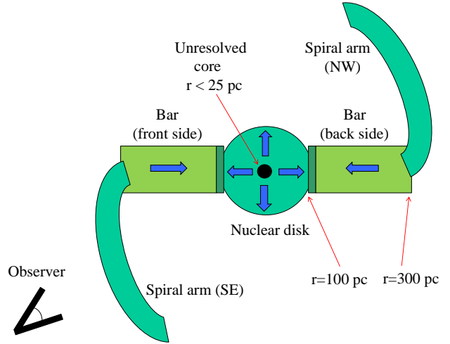
Fig. 26. A sketch of the central parts of NGC 4945 viewed from a position above the plane and on top of the center of the galaxy. The blue arrows indicate modeled or observationally suggested radial motions of the gas.
