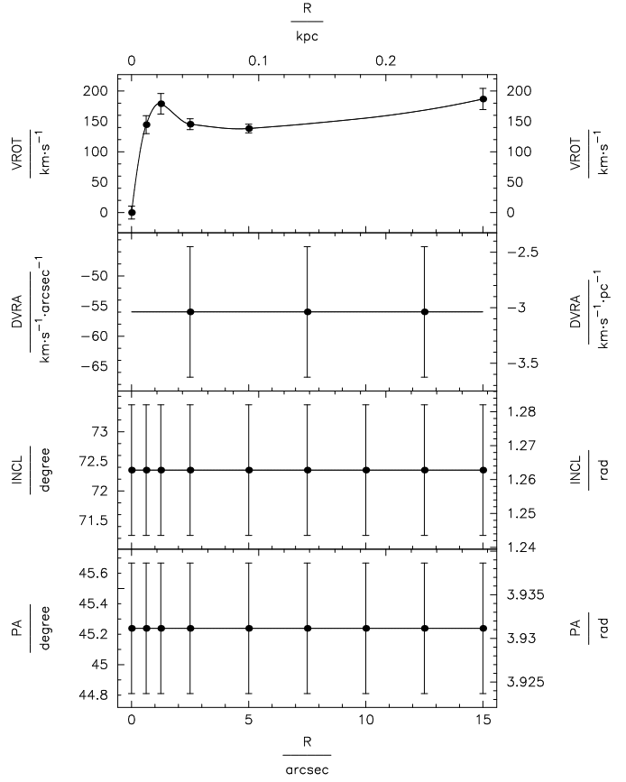
Fig. 19. Final parametrisation (from top to bottom): Rotation velocity, vertical velocity gradient DVRA (see Sect. 4.6.2), inclination, and position angle as a function of galactocentric radius. These are the parameters, which are assumed to be shared by all the lines included in Figs. 18, 20, 21 and 23.
