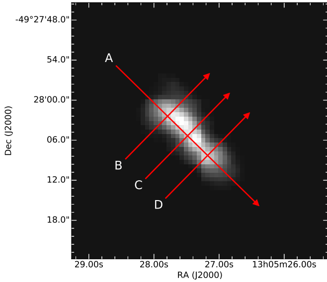
Fig. 22. Slice positions of PV-diagrams in Fig. 23 overlaid on a velocity integrated intensity map of the \text{CH}_3\text{C}_2\text{H} 5_0 \rightarrow 4_0 line (see, e.g., Table 1 and Fig. 4.) The PV-diagrams in Fig. 23 are all directed from left (east) to right (west).
